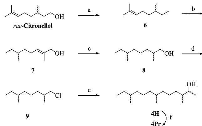
Scheme 5. a) 1. p\text{TsCl} , pyridine, 2. \text{LiAlH}_4 , \text{Et}_2\text{O} ; b) 1. t\text{BuOOH} , \text{SeO}_2 , 2. \text{NaBH}_4 ; c) \text{Raney Ni} , \text{H}_2 , \text{MeOH} , 40^\circ\text{C} ; d) \text{PPh}_3 , \text{CCl}_4 , reflux; e) 1. \text{Li(s)} , reflux, n -hexane, 2. addition to a cis/trans mixture (58:42) of rac -3,4-dimethyl- \gamma -butyrolactone at -78^\circ\text{C} , 3. \text{N}_2\text{H}_4 \times \text{H}_2\text{O} , \text{KOH} , diethylene glycol, 170^\circ\text{C} , 1 h, then 210^\circ\text{C} , 3 h; f) 10 equiv. \text{CH}_3\text{CH}_2\text{COCl} , \text{CH}_2\text{Cl}_2
