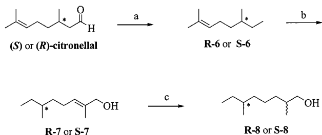
Scheme 1. a) N 2 H 4 × H 2 O, KOH, diethylene glycol, 170 °C; b) 1. t BuOOH, SeO 2 , CH 2 Cl 2 , 2. NaBH 4 , NaOH, MeOH, 0–30 °C; c) Raney Ni, H 2 , MeOH, 40 °C
