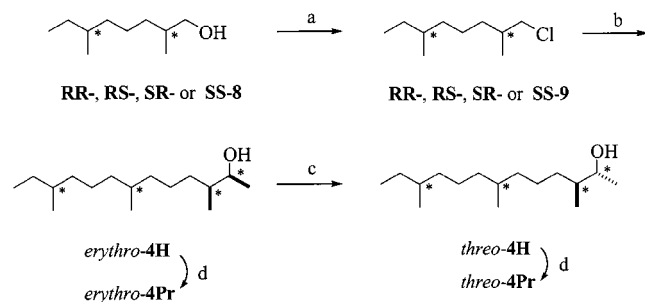
Scheme 4. a) \text{PPh}_3 , \text{CCl}_4 , reflux; b) 1. \text{Li(s)} , reflux, n -hexane, 2. addition to one of the enantiomers of cis -3,4-dimethyl- \gamma -butyrolactone at -78^\circ\text{C} , 3. \text{N}_2\text{H}_4 \times \text{H}_2\text{O} , \text{KOH} , diethylene glycol, 170^\circ\text{C} , 1 h, then 210^\circ\text{C} , 3 h; c) 1. \text{PPh}_3 , \text{PhCO}_2\text{H} , \text{N}_2(\text{CO}_2\text{Et})_2 , 2. \text{NaOH} , \text{H}_2\text{O}/\text{MeOH}/\text{dioxane} ; d) 10 equiv. \text{CH}_3\text{CH}_2\text{COCl} , \text{CH}_2\text{Cl}_2
