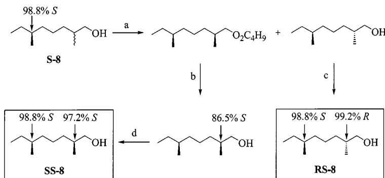
Scheme 2. a) Lipase-catalysed kinetic acylation; Amano PS, CHCl 3 , vinyl butyrate, a_w \approx 0 , c = 50\% and then LC separation of the product and the substrate; b) KOH/MeOH; c) lipase-catalysed kinetic acylation; Amano PS, CHCl 3 , vinyl butyrate, a_w \approx 0 , c = 60\% and then LC separation of the product and the substrate; d) 1. lipase-catalysed kinetic acylation; Amano PS, CHCl 3 , vinyl butyrate, a_w \approx 0 , c = 51\% and then LC separation of the product and the substrate; 2. KOH/MeOH
