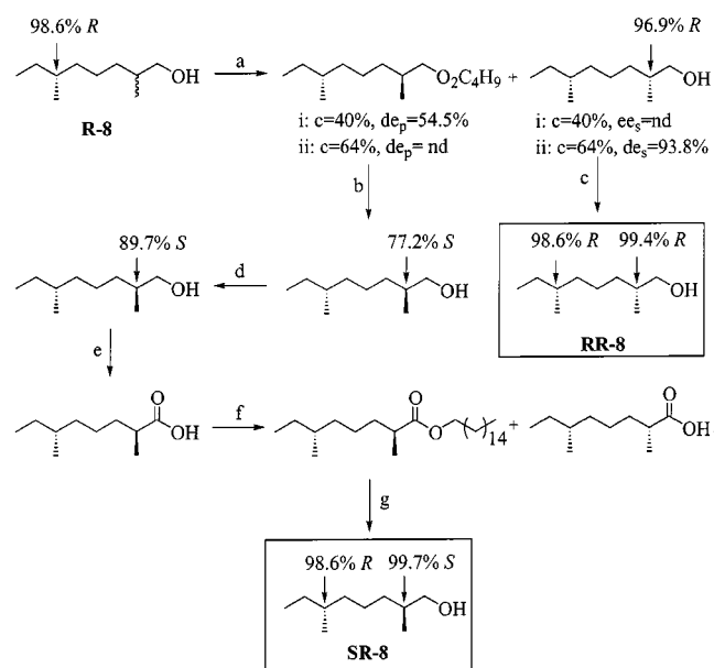
Scheme 3. a) Lipase-catalysed kinetic acylation; Amano PS, CHCl 3 , vinyl butyrate, a_w \approx 0 , c = 40\% or 64\% and then LC separation of the product and the substrate; b) KOH/MeOH; c) substrate ii, lipase-catalysed kinetic acylation; Amano PS, CHCl 3 , vinyl butyrate, a_w \approx 0 , c = 40\% and then LC separation of the product and the substrate; d) 1. lipase-catalysed kinetic acylation; Amano PS, CHCl 3 , vinyl butyrate, a_w \approx 0 , c = 70\% and then LC separation of the product and the substrate; 2. KOH/MeOH; e) CrO 3 /H 2 SO 4 acetone, 0 °C; f) lipase-catalysed kinetic acylation; Im-CRL, 1-hexadecanol, a_w \approx 0.8 , cyclohexane, c = 40\% ; g) LiAlH 4 , Et 2 O
